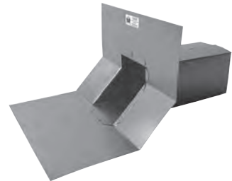
Scupper Outlets
